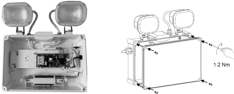
Figure 2: Showing internal layout and battery plug to be connected at arrow point.
